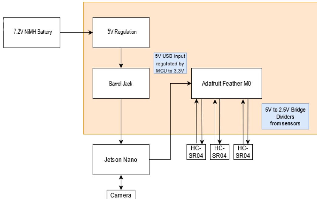
Figure 16: Power management system on PCB
