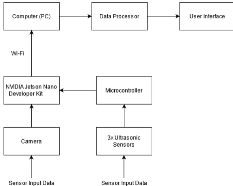
Figure 10: Block diagram for 3D scanning device
