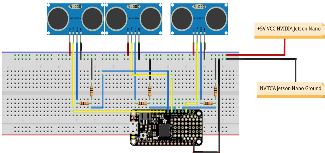
Figure 12: Breadboard diagram of Ultrasonic Subsystem
