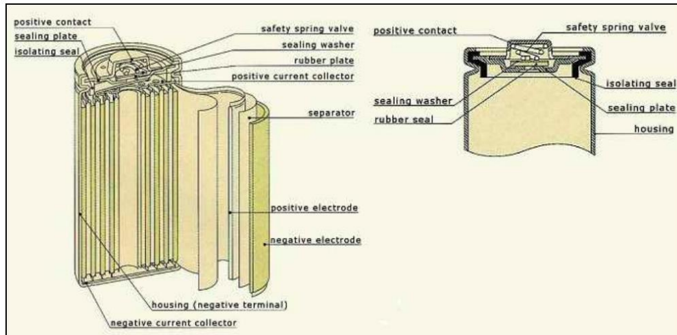
Figure 6: Design of a Rechargeable Battery
