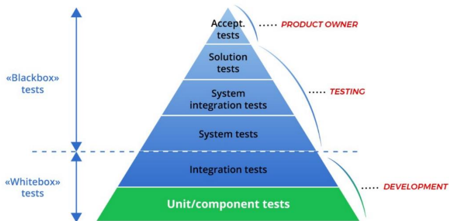
Figure 19: Software Testing
